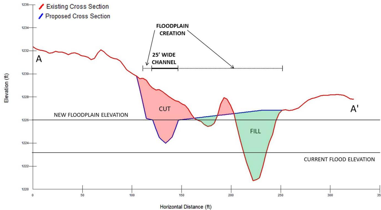
Kingsbury Creek: Current vs Concept Stream Cross Section
